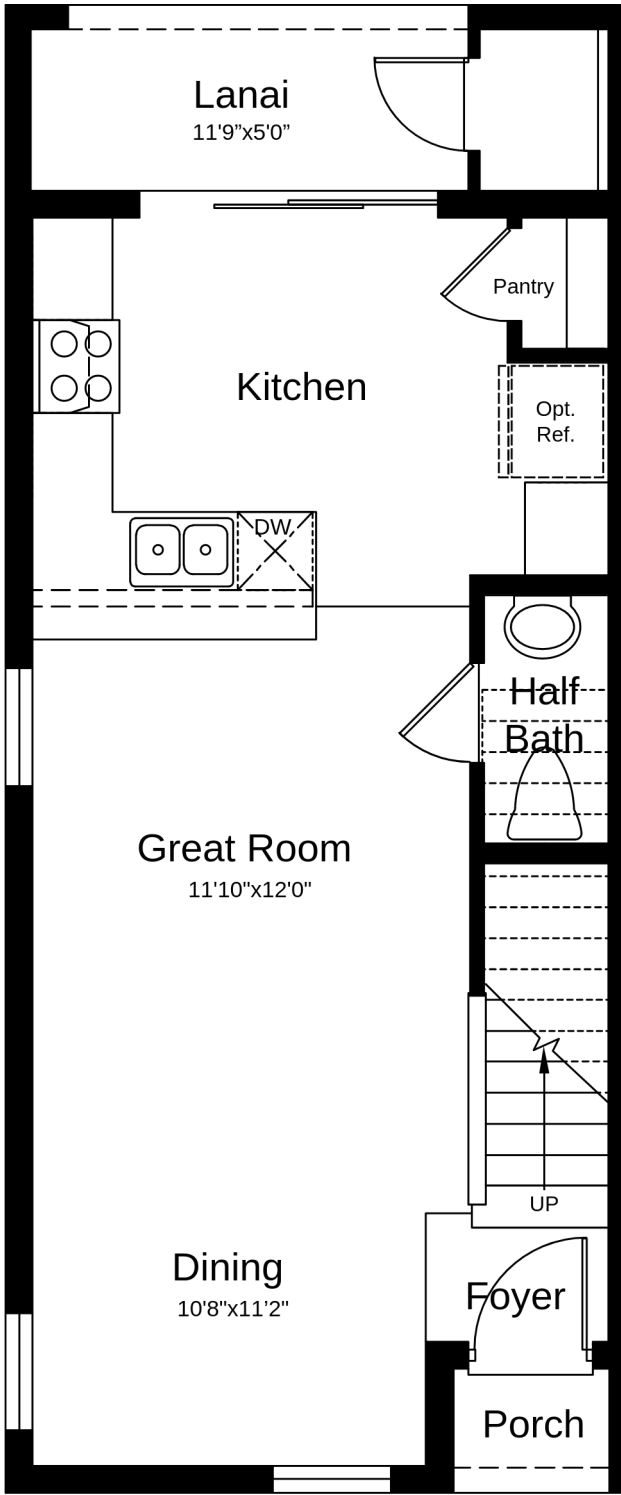
Floor 1
